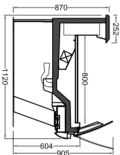
NEVA112-YY-S BLOK AVAK NEVA112-YY-S WITH LEGS
