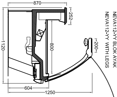
NEVA122-YY BLOK AVAK NEVA122-YY WITH LEGS
