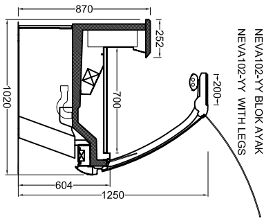
NEVA112-YY BLOK AVAK NEVA112-YY WITH LEGS
