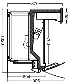
NEVA102-YY-S BAZALI NEVA102-YY-S COVERED BASE
