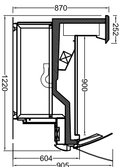
NEVA122-YY-S BAZALI NEVA122-YY-S COVERED BASE
