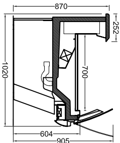
NEVA102-YY-S BLOK AVAK NEVA102-YY-S WITH LEGS
