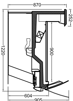
NEVA122-YY-S BLOK AVAK NEVA122-YY-S WITH LEGS
