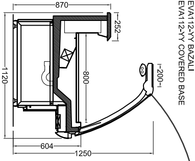
NEVA122-YY BAZALI NEVA122-YY COVERED BASE
