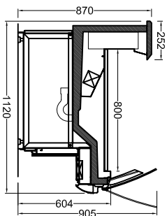
NEVA112-YY-S BAZALI NEVA112-YY-S COVERED BASE
