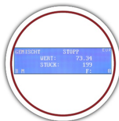
Printing function
