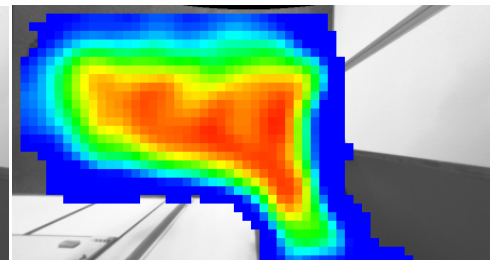
Heat Map
